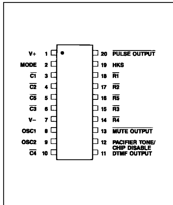
Figure 1 : Pin Connection.
